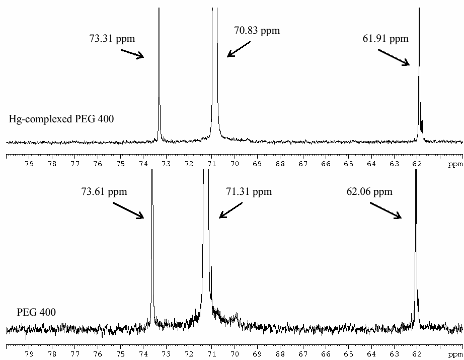
Figure 15. Overlay of PEG 400 and Hg-complexed PEG 400 ^{13}\text{C} -NMR spectra.
