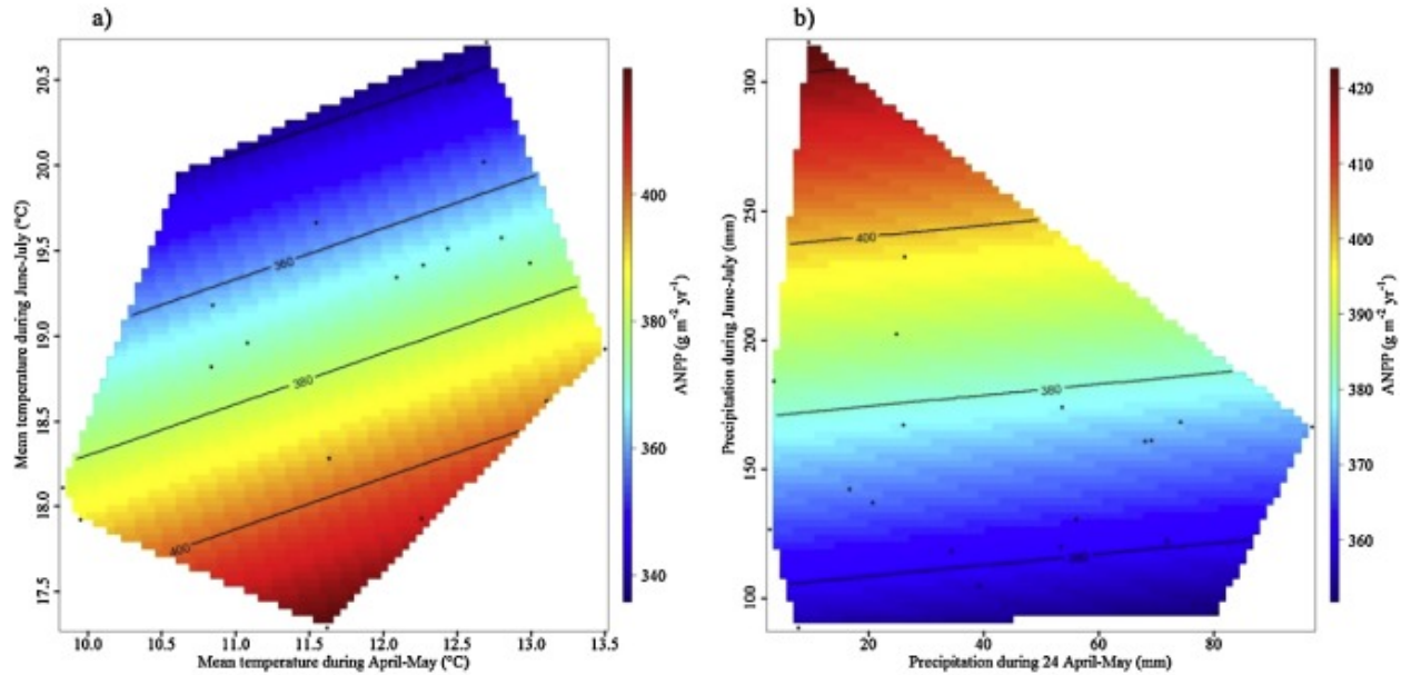
Figure 2. Grassland productivity at Yunwushan as a function of (a) temperature and (b) precipitation during both spring (April–May for temperature analysis and 24 April–May for precipitation analysis since consistently negative impacts of precipitation occurred after 24 April until the end of May in Fig. 1; x-axis) and summer (June–July, y-axis). Variation in color reflects variation in ANPP, while the black dots indicate the annual productivity records between 1992 and 2011.
