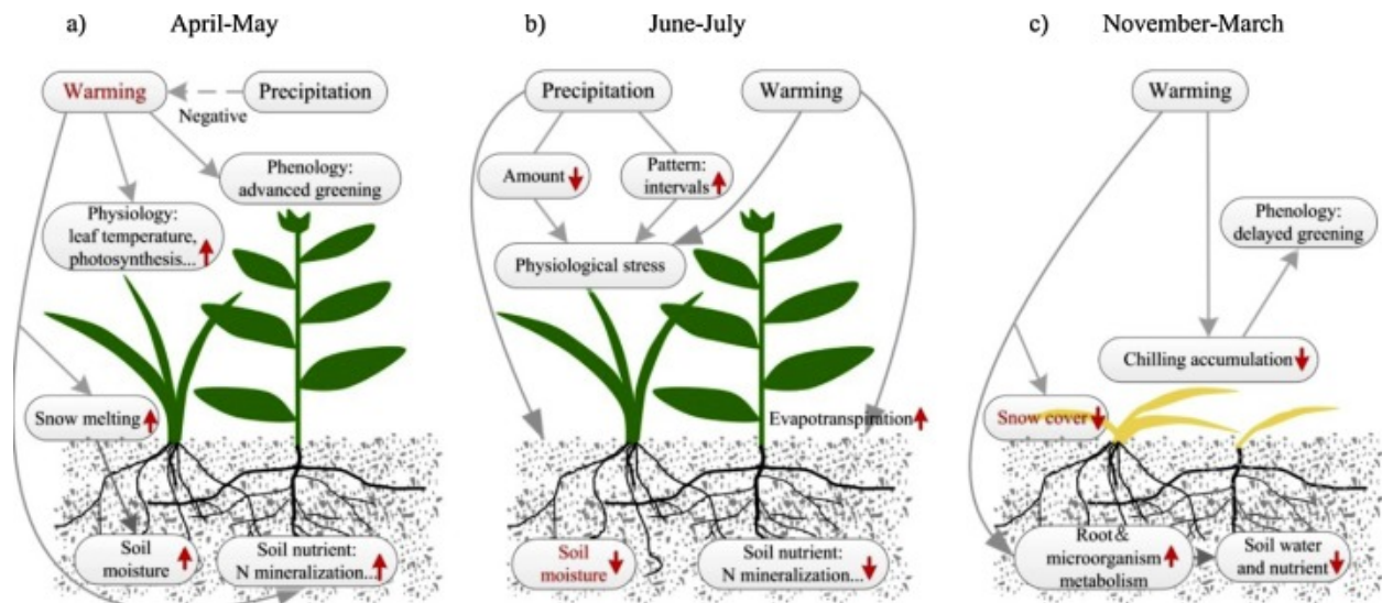
Figure 4. Potential relationships between grassland productivity and climate variability during (a) April–May, (b) June–July and (c) November–March at Yunwushan.
