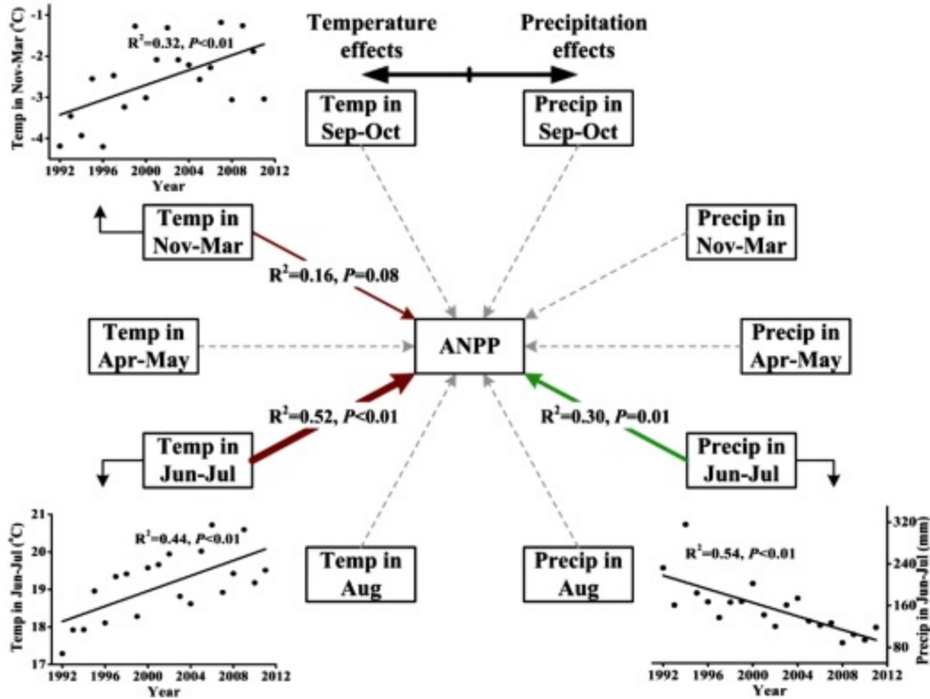
Figure 3. Relationships between grassland productivity and mean temperature and precipitation for different periods during 1992–2011 at Yunwushan. Trends of temperature during November–March and June–July, as well as precipitation during June–July are shown in the inset plots. Red arrows indicate significant negative correlations between grassland productivity and climate variables, while green arrows mean significant positive relationships. The dashed lines imply that no significant correlations were detected between ANPP and climate variation during these periods.
