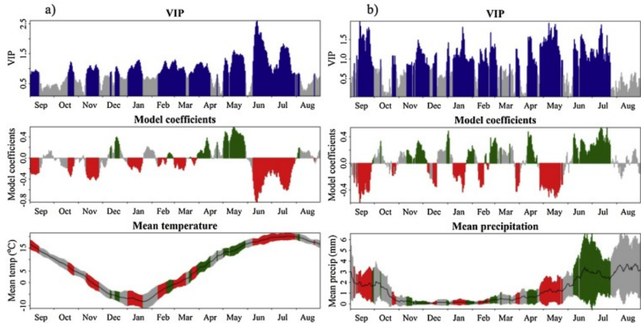
Figure 1. Results of Partial Least Squares (PLS) regression correlating grassland productivity at Yunwushan during 1992–2011 with 15-day running means of (a) daily mean temperature and (b) daily precipitation from previous September to August. Blue bars in the top row indicate that VIP values are greater than 0.8, the threshold for variable importance. In the middle row, red color means model coefficients are negative and important, while green color indicates important positive relationships between grassland productivity and climate variables. The black lines in the bottom panel stand for daily mean temperature and precipitation, while grey, green and red areas represent the standard deviation of daily climate variables.
