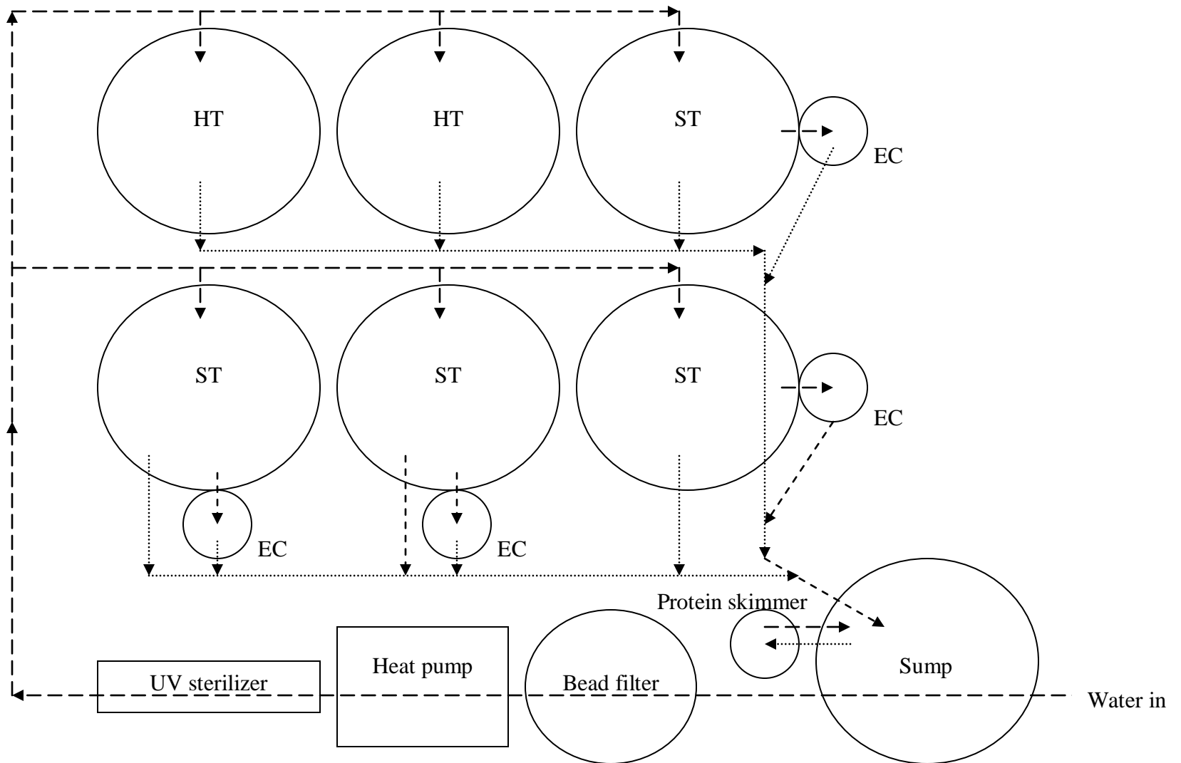
Figure 1. Layout of the black sea bass broodstock system (not to scale). Arrows depict water flow through the recirculating system (water in \rightarrow ), (water out \cdots\rightarrow ). HT = holding tank, ST = Spawning tank, EC = egg collector.
