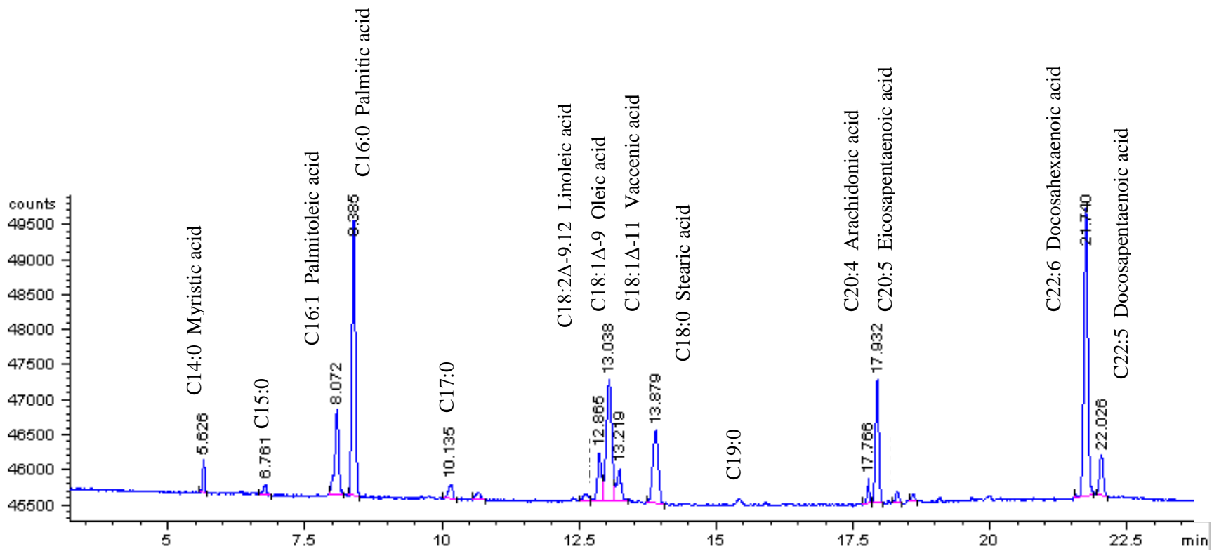
Figure 17. GC-FID chromatogram of FAMES produced from a black sea bass egg sample.
