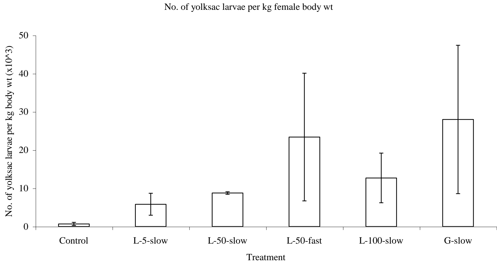
Figure 12. No. of yolksac larvae per kg female body wt ( \times 10^3 ) under different hormone treatments. Data represent means \pm standard error ( N = 6-21 ). Letter indicates hormone (L = LHRH-a, G = GnRH-a), number indicates dose ( \mu\text{g}/\text{kg} ), and word indicates release rate (slow or fast). No significant ( P > 0.05 ) differences among treatments were observed.
