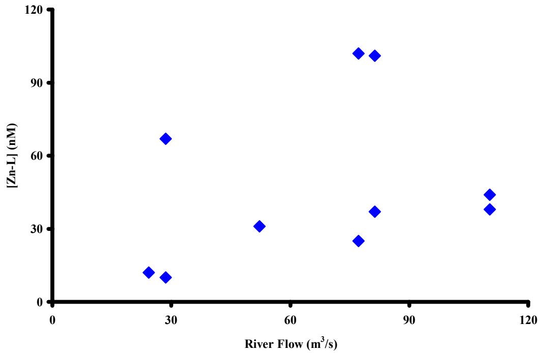
Figure 7. Relationship between (a) TDZn and (b) Zn-complexing ligands and river flow from bottom waters at both sampling stations at all sampling times. Both plots show no statistical significance ( p > 0.05 ).
