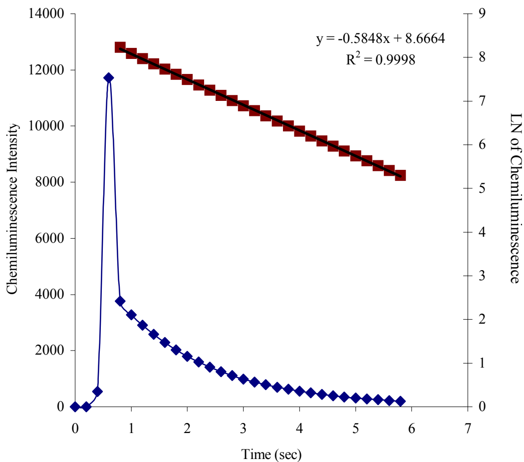
Rate Constant for Chemiluminescence Emission Decay for Chamber 6
