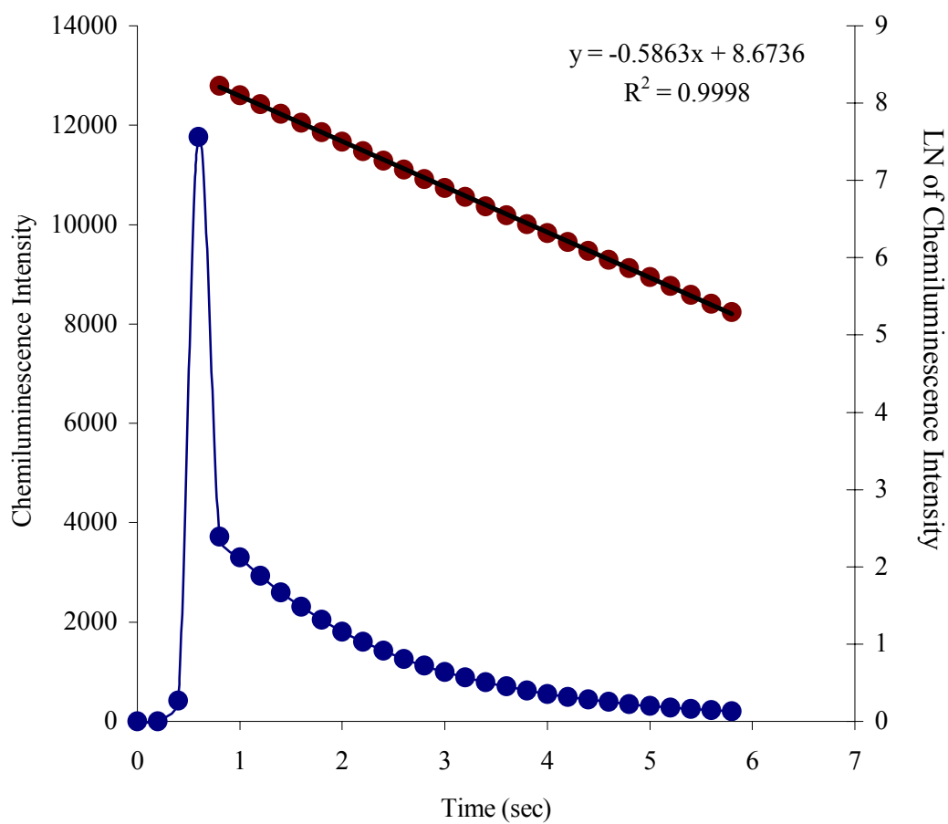
Rate Constant for Chemiluminescence Emission Decay for Chamber 4
