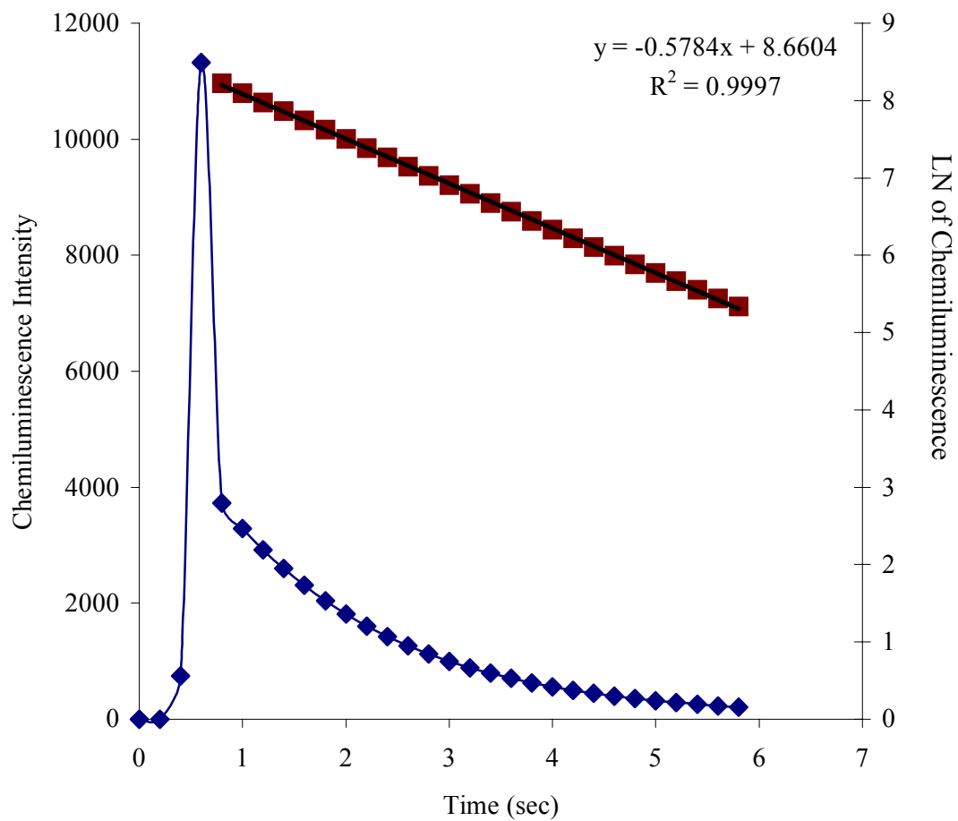
Rate Constant for Chemiluminescence Emission Decay for Chamber 2
