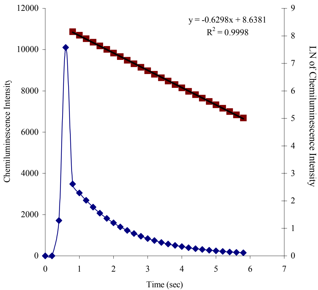
Rate Constant for Chemiluminescence Emission Decay for Chamber3
