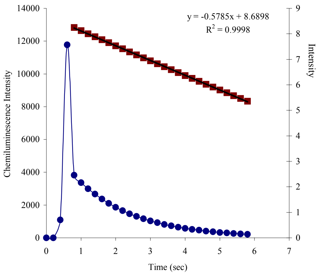
Rate Constant of Chemiluminescence Emission Decay for Chamber 1
