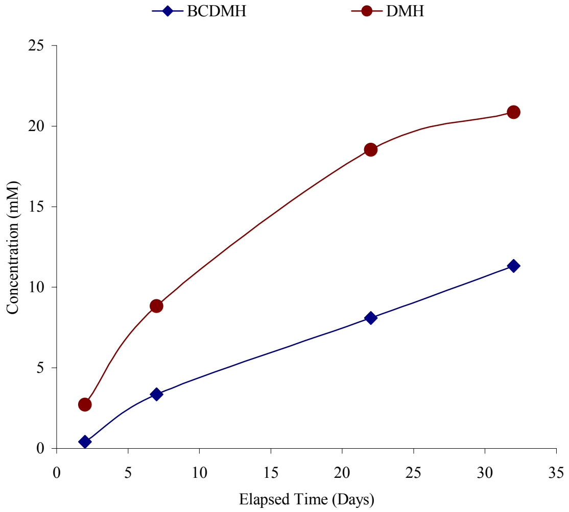
Plot of BCDMH and DMH Concentrations in Chamber 2
