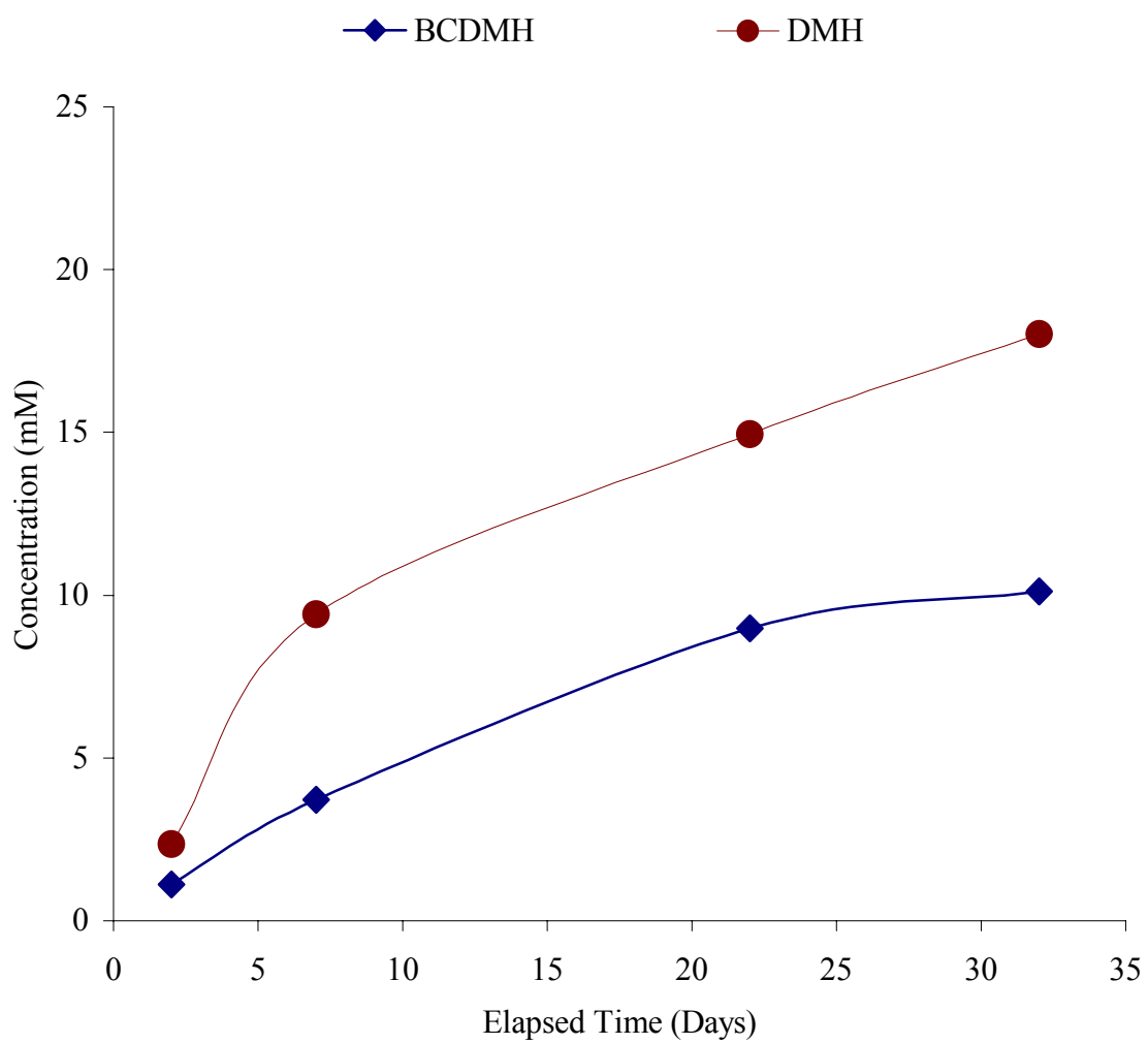
Plot of BCDMH and DMH concentrations in Chamber 3
