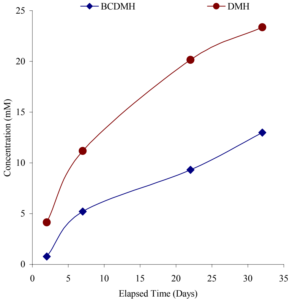
Plot of BCDMH and DMH Concentrations in Chamber 7
