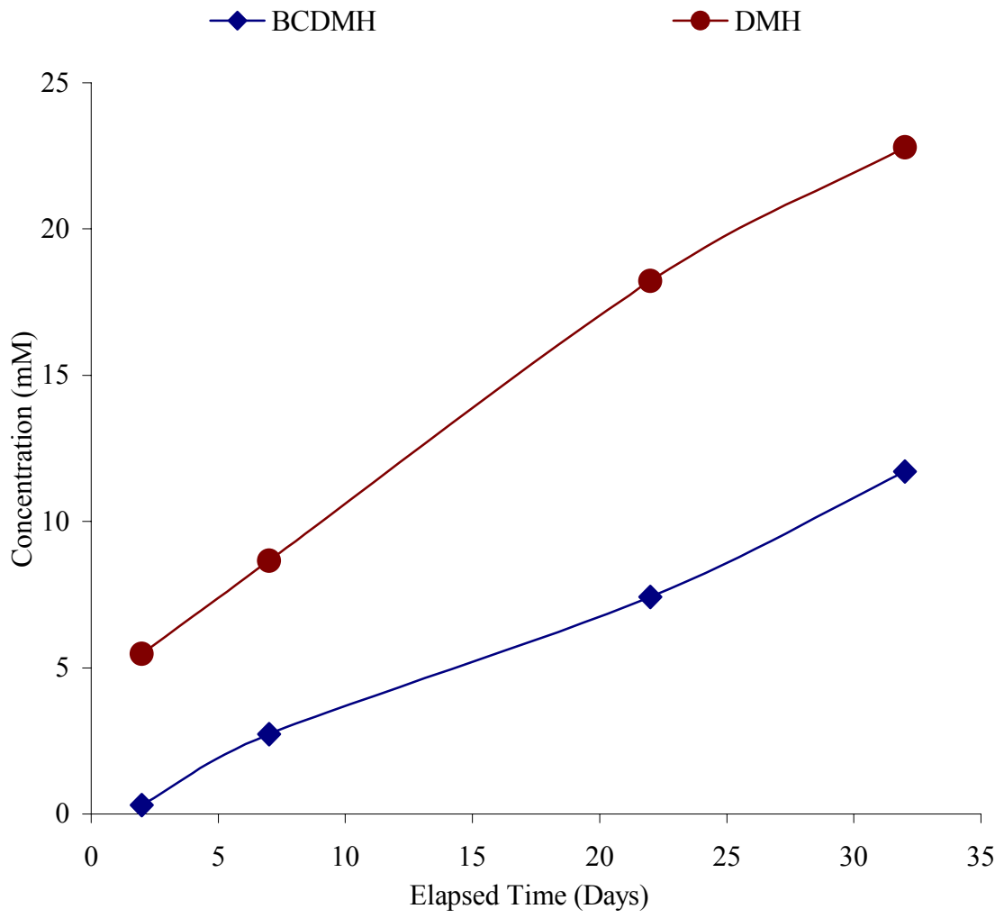
Plot of BCDMH and DMH Concentrations in Chamber 8
