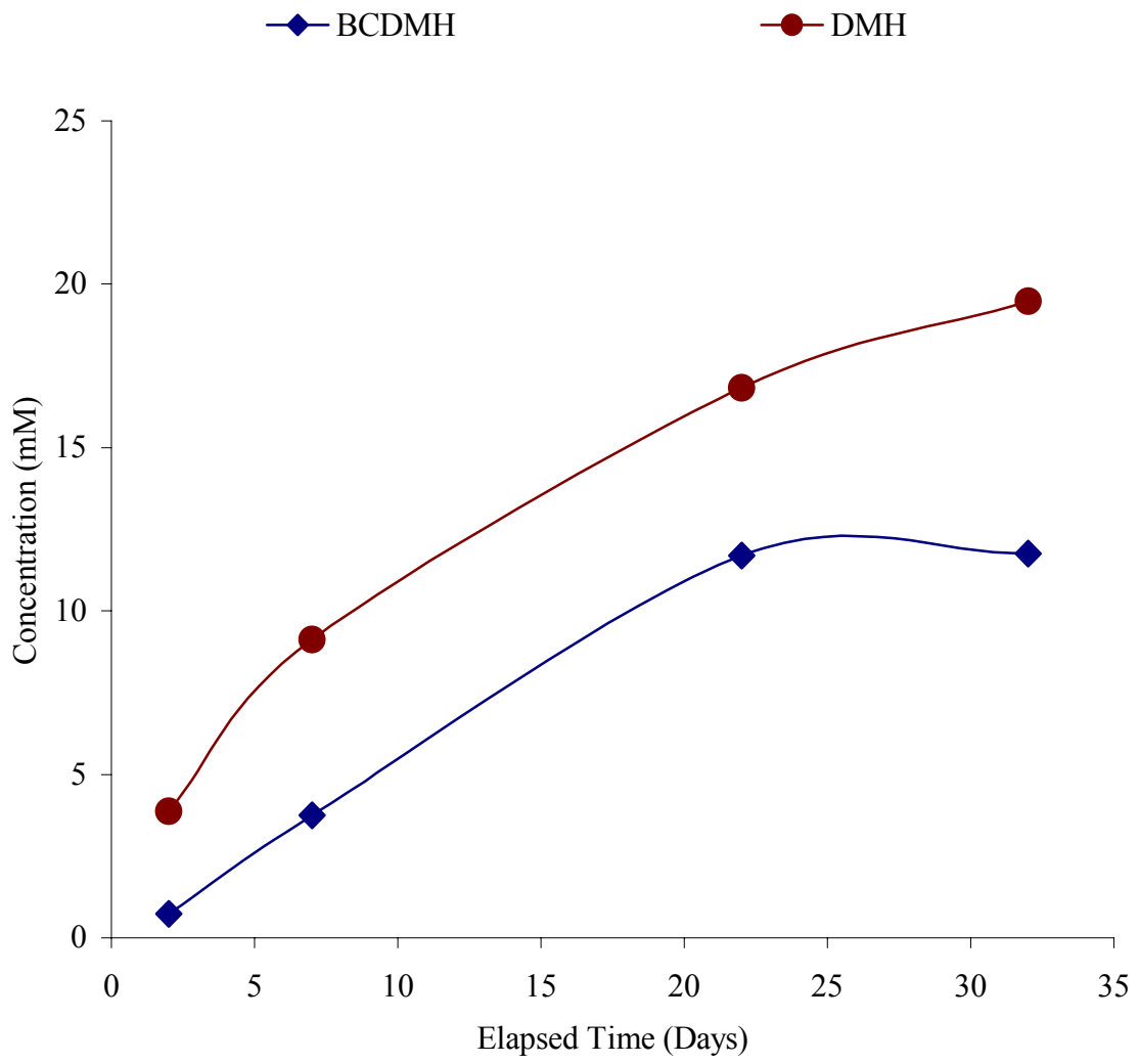
Plot of BCDMH and DMH Concentrations in Chamber 4
