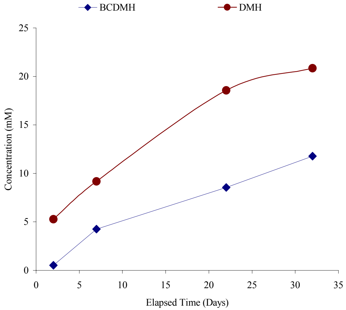
Plot of theBCDMH and DMH concentrtaions in Chamber 1
