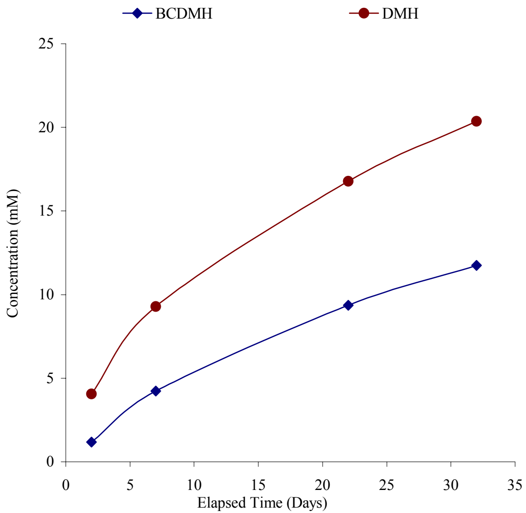
Plot of BCDMH and DMH Concentrations in Chamber 5
