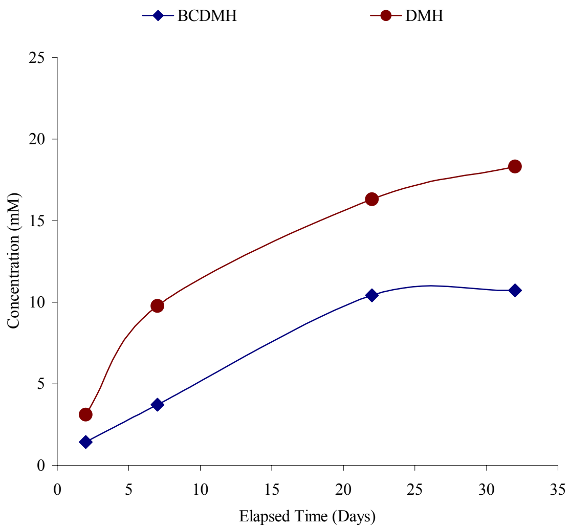
Plot of BCDMH and DMH Concentrations in Chamber 10
