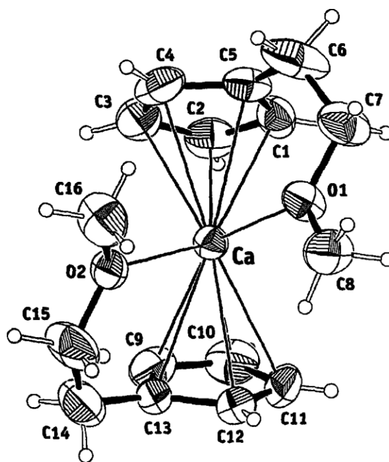
Fig. 2. ORTEP diagram of (\text{Cp}^{\text{s}})_2\text{Ca} , illustrating the numbering scheme used in the text. Thermal ellipsoids are shown at the 30% level.
