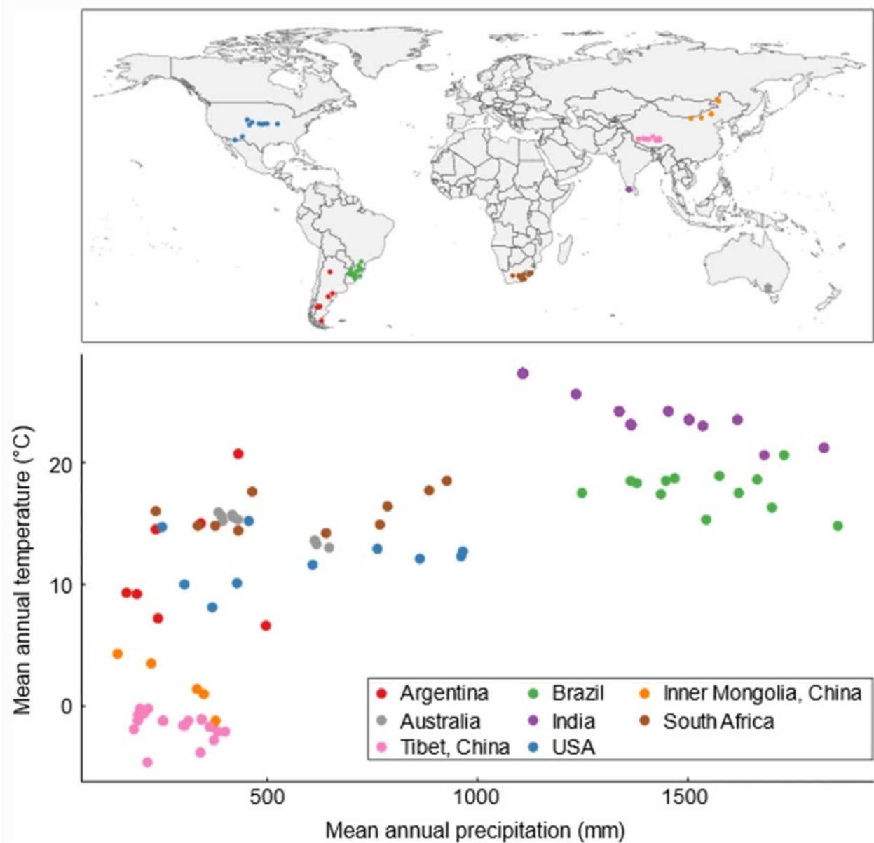
Fig. 2 a Location of the eight water availability gradients in grassy biomes on five continents. b Mean annual precipitation (MAP) and temperature (MAT) parameter space encompassed by the study sites.
