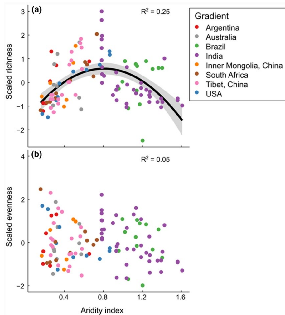
Fig. 3 Relationship between plant species a richness, b evenness and water availability (Aridity Index) among grassy biome sites globally. Quadratic models were fitted to the data and R2 values are reported, with the regression line only shown for significant models. Grey shading indicates the 95% confidence interval. There were 115 datapoints in this analysis.
