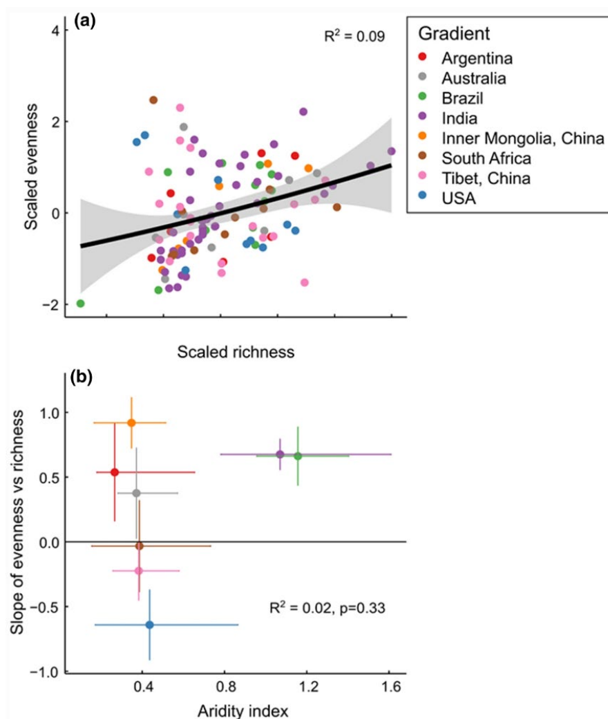
Fig. 4 a Relationship between plant species richness and evenness among grassy biome sites globally. Grey shading indicates the 95% confidence interval. b Relationship between the slope of the relationship between species richness and evenness and water availability (Aridity Index). There were 115 datapoints in this analysis. The x-axis is the geometric mean of the aridity gradient for each biome and the x-error bars are the minimum and maximum aridity values for each biome. The y-error bars are the error in the slope estimates from the linear regression models.
