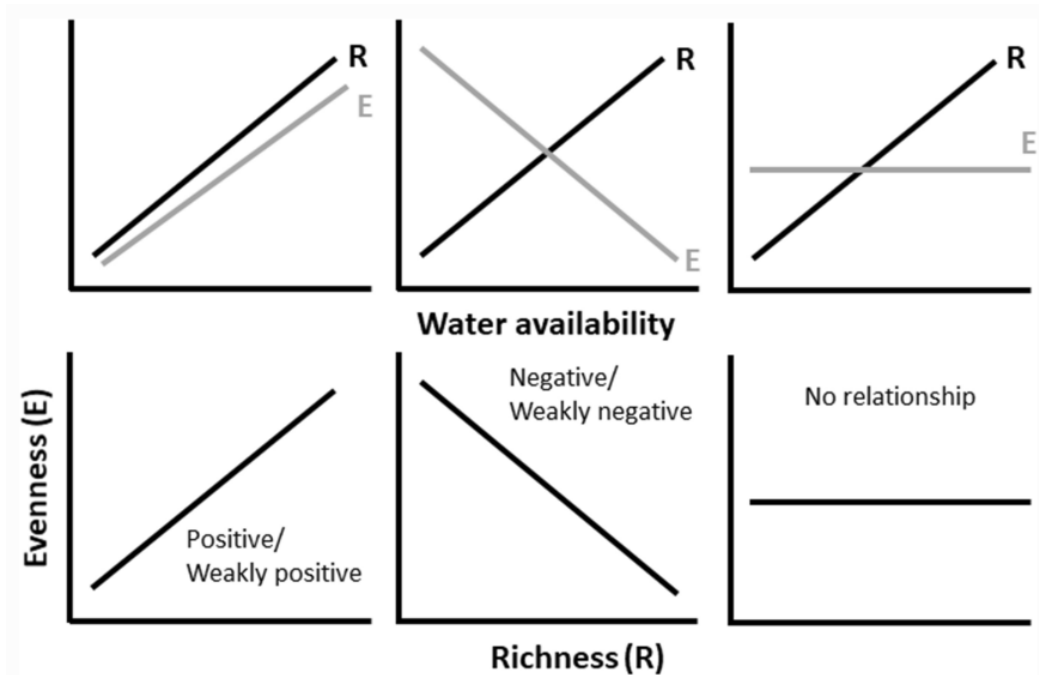
Fig. 1 Conceptual figure hypothesizing possible relationships between water availability (aridity or precipitation) and richness (R) and evenness (E). It is expected that if richness is primarily abiotically constrained at broad spatial scales, then it should be positively related to water availability. Much less is known about the spatial relationship between water availability and evenness, and a positive, negative, or no relationship are possible. As a consequence, when considering the relationship between richness and evenness, a negative, positive, or no relationship may be expected to result.
