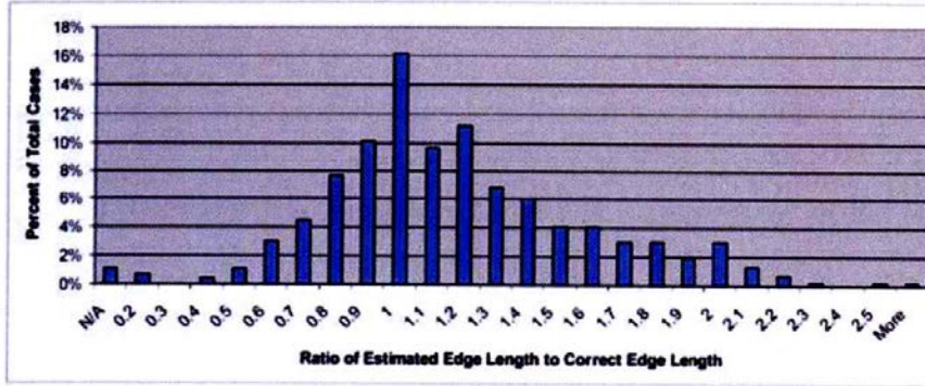
Figure 4: Correctness of the edge length bias estimate for large graphs ( N = 100 ).
