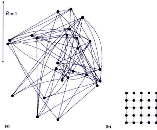
Figure 2: (a) Spatial random graph generated with N = 25 , R = 1 , H = 0.25 , p + p_b = 0.5 , P-\Delta = 0.25 . The estimated neighborhood radius was \sigma = 0.247 , and bias \beta = 0.777 ; (b) Square lattice with 25 vertices.
