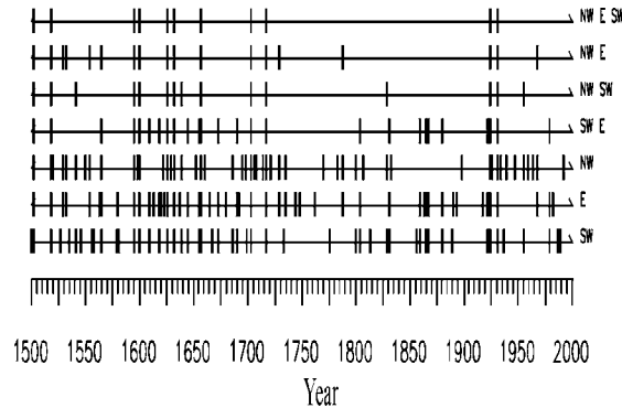
FIG. 2. Temporal occurrence of extreme climatic pointer years by super-region (NW E SW), region (NW E, NW SW, and SW E), and subregion (NW, E, and SW).
