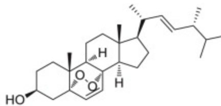
Ergosterol peroxide (2)
