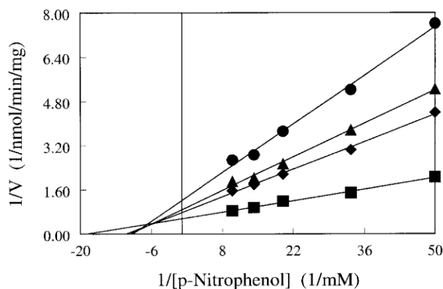
Fig. 1. Inhibition of rabbit liver microsome-catalyzed p -nitrophenol oxidation by farnesol. The concentration of farnesol in each of the experiments was (■) 0 \mu\text{M} , (◆) 45 \mu\text{M} , (▲) 90 \mu\text{M} , and (●) 180 \mu\text{M} .
