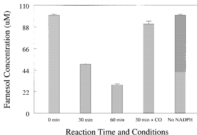
Fig. 2. Time-dependent metabolism of farnesol in rabbit liver microsomes in the presence of NADPH. Also shown are the results of identical reactions in the absence of NADPH after a 60-min incubation, and in the presence of CO after a 30-min incubation. Reactions were terminated by addition of ethyl acetate, and samples were analyzed by GC/MS and signals normalized using the internal standard 6-phenylhexanol.
