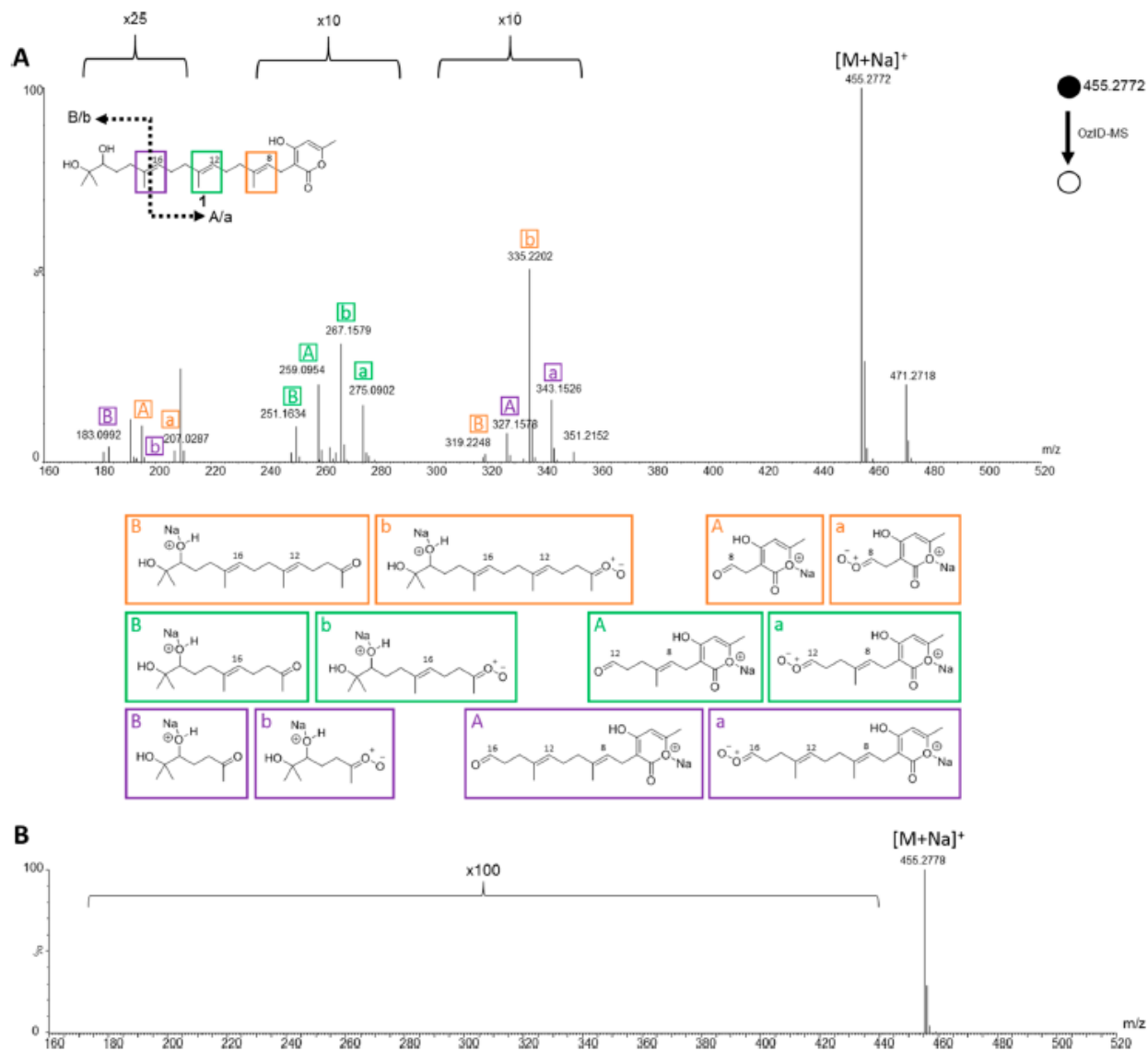
Figure 3. (A) OzID-MS spectrum of ent -sartorypyrone E ( 1 ) after targeted OzID fragmentation. The structure of 1 is shown on the top left. The purple, green, and orange boxes around the diterpene double bonds indicate positions where ozonolysis occurred. The informative OzID fragments are labeled with the colors corresponding to the structure. The capital letters represent the ketone fragments, and the lower-case letters represent the Criegee ion fragments. The A/a corresponds to the sodium ion associating with the lactone ring (right side of the molecule), whereas the B/b corresponds to the sodium ion associating with hydroxys at the end of the isoprene chain (left side of the molecule). The OzID-MS products (shown under spectrum) are color and letter coded to represent the cleaved double bond, and these data are tabulated in Supporting Information Table S2. (B) Compound 1 being analyzed in argon, to demonstrate that the fragments in A are unique to OzID-MS
