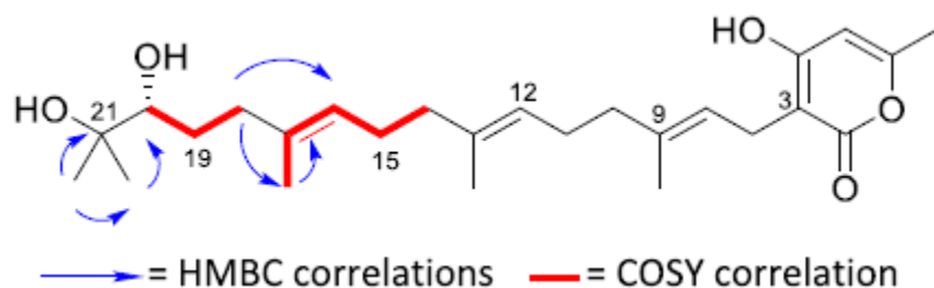
Figure 2. Key COSY and HMBC correlations for compound 1 .
