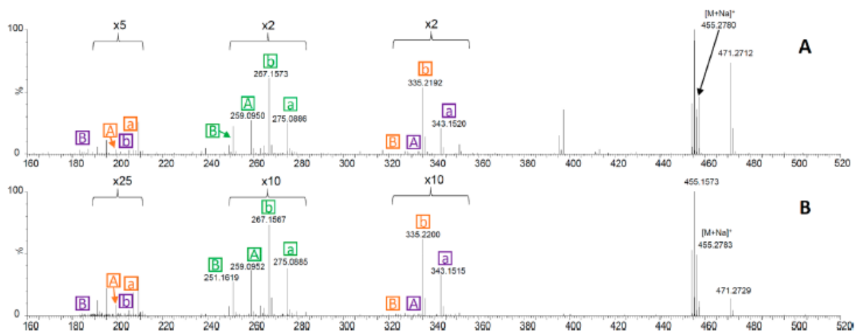
Figure 8. OzID-MS studies of Aspergillus fischeri showing the analysis of compound 1 in the context of an extract (panel A) and from in situ sampling of a Petri dish of a live culture (panel B). The fragmentation patterns in both cases are analogous to those in Figure 3, and these data are tabulated in Supporting Information Tables S3 and S4.
