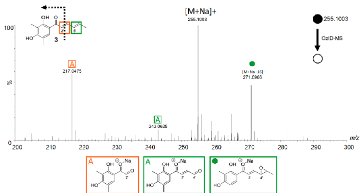
Figure 5. OzID-MS spectrum of 3 after targeted OzID fragmentation. The structure of 3 is shown on the top left. The green and orange boxes around the double bonds indicate positions where ozonolysis occurred. The informative OzID fragments are labeled with the colors corresponding to the structure, analogous to those in Figure 3. The OzID-MS products (shown under spectrum) are color and letter coded to represent the double bond that was cleaved, and these data are tabulated in Supporting Information Table S6.
