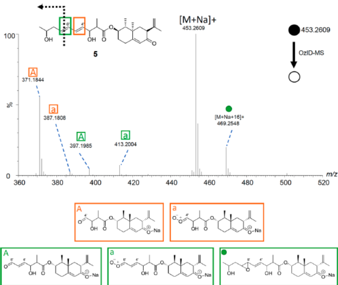
Figure 7. OzID-MS spectrum of 5 after targeted OzID fragmentation. The structure of 5 is shown on the top left. The green and orange boxes around the double bonds indicate positions where the ozonolysis occurred. The informative OzID fragments are labeled with the colors corresponding to the structure, analogous to those in Figure 3. The OzID-MS products (shown under spectrum) are color and letter coded to represent the double bond that was cleaved, and these data are tabulated in Supplementary Table S8.
