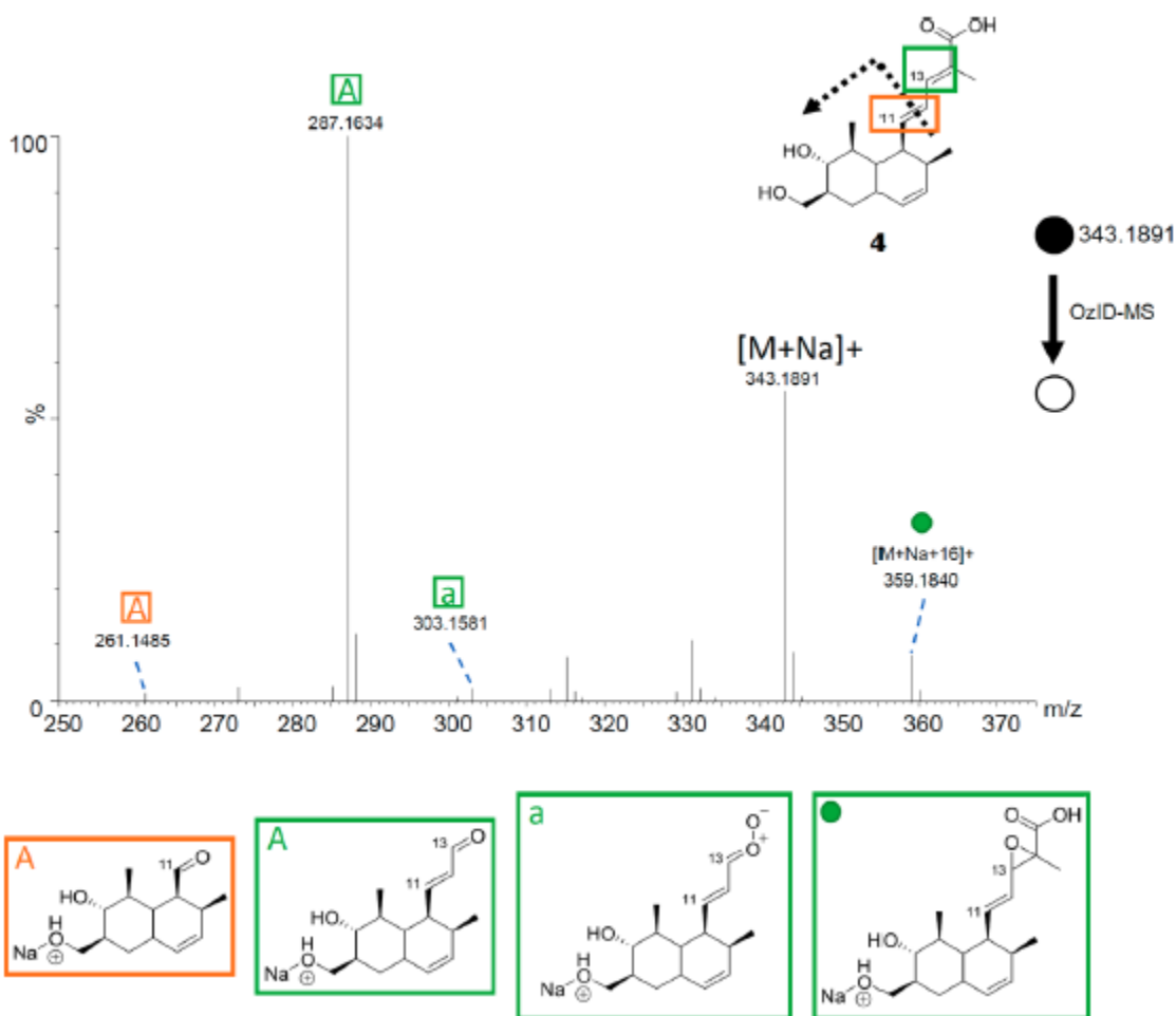
Figure 6. OzID-MS spectrum of 4 after targeted OzID fragmentation. The structure of 4 is shown on the top left. The green and orange boxes around the double bonds indicate positions where ozonolysis occurred. The informative OzID fragments are labeled with the colors corresponding to the structure, analogous to those in Figure 3. The OzID-MS products (shown under spectrum) are color and letter coded to represent the double bond that was cleaved, and these data are tabulated in Supporting Information Table S7.
