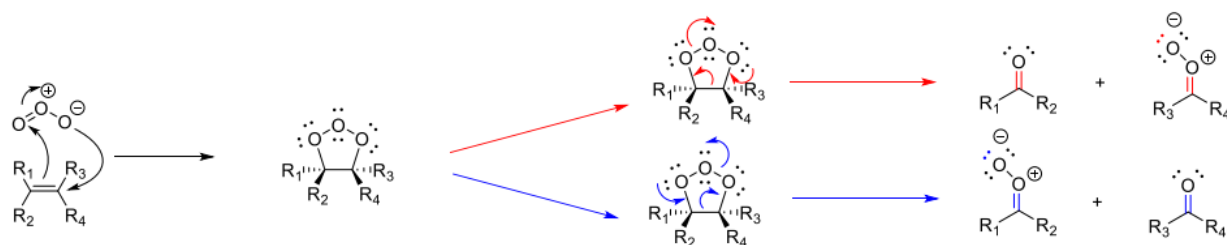
Figure 1. In ozonolysis carbon–carbon double bonds react with ozone via a 1,3-dipolar cycloaddition. Two products are formed via the subsequent retro-1,3-dipolar cycloaddition, resulting in a ketone/aldehyde and a Criegee intermediate. The red arrows (top) and blue arrows (bottom) represent the two routes in which the molozonide can undergo the retro-1,3-dipolar cycloaddition.
