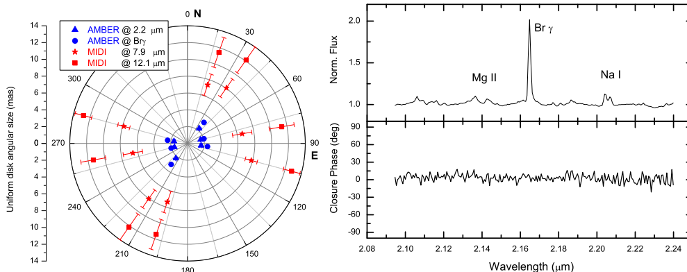
Figure 3. Left: Uniform disk sizes dependence on the baseline position angle (in degrees) for 2 selected wavelengths both from AMBER (continuum at 2.2 \mu\text{m} and center of the \text{Br}\gamma line) and from MIDI ( 7.9 \mu\text{m} and 12.1 \mu\text{m} ). The central star is supposed to be at the center of the plot and the distance between 2 symmetrical points gives the corresponding uniform disk angular diameter ( \theta_{\text{UD}} ) of the CSE. The error bars on the AMBER \theta_{\text{UD}} have similar sizes as their corresponding symbols. Although the \theta_{\text{UD}} is a zero-order estimate, this figure allows us to directly compare the CSE sizes in the near- and mid-IR. Right: VLTI/AMBER closure phase for CPD-57° 2874 obtained around \text{Br}\gamma with R = 1500 . Within the noise level ( \simeq \pm 10^\circ ) the closure phase is zero (continuum and \text{Br}\gamma line) suggesting a centrally-symmetric intensity distribution in the near-IR. Spherical and non-spherical (with axial-symmetry) CSEs are thus compatible with the zero closure phase measured with AMBER.
