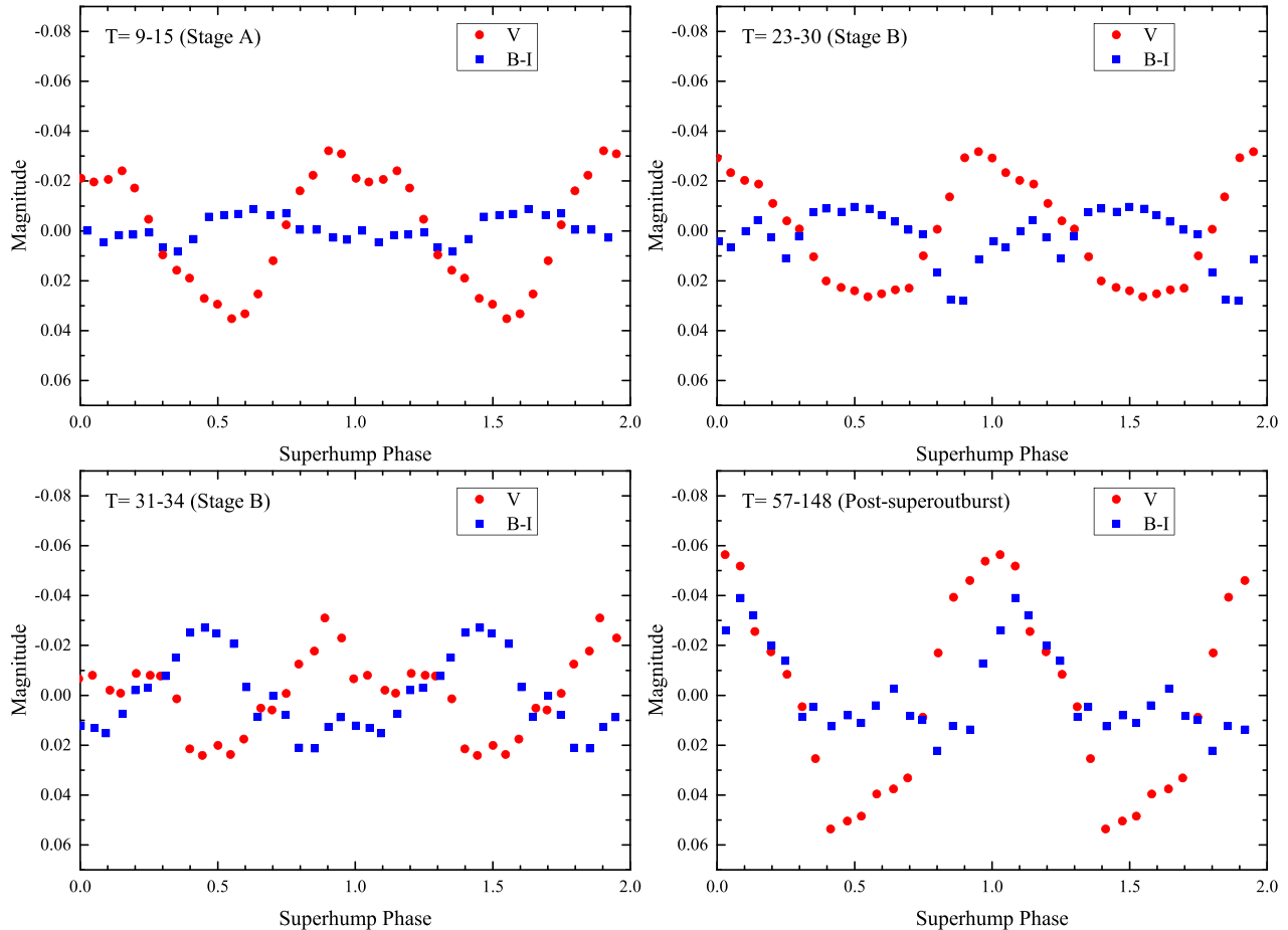
Figure 9. Phase-averaged V light curves and B-I colour variations of superhumps at different stages of the superoutburst of SSS J122222.
