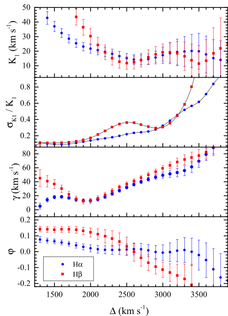
Figure 16. The diagnostic diagram for the H \alpha and H \beta emission lines from the T = 72 observations, showing the response of the fitted orbital elements to the choice of the double-Gaussian separation.
