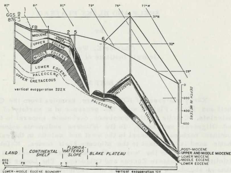
Figure 1. Isometric fence diagram showing the stratigraphy of the Continental Margin of the east coast of Florida. From JOIDES (1965).
