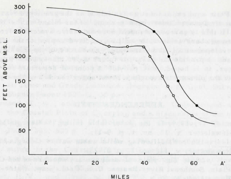
Figure 3. Original and 1942 hydrologic profile along A-A' of Figure 2. The original profile (solid points) is from Figure 1, the 1942 profile (open points) from Warren (1944). The 1942 profile crosses the edge of the 1942 recharge plateau twice and therefore is slightly saddled, it should be interpreted as a smooth curve. The average decline in the hydrologic profile from 1880 to 1942 was approximately 50 feet.
