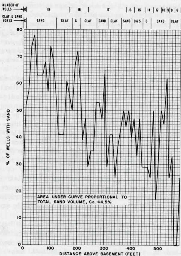
Figure 2. Distribution of sands within the Potomac Formation.
