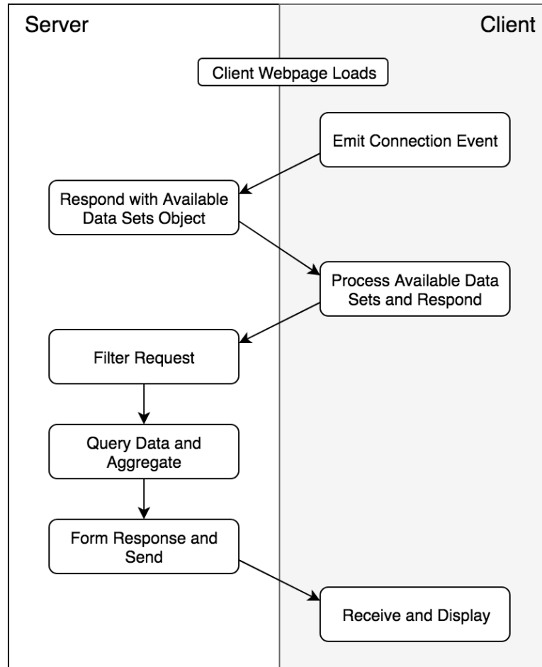
Figure 5.3: Server-Client Handshake
